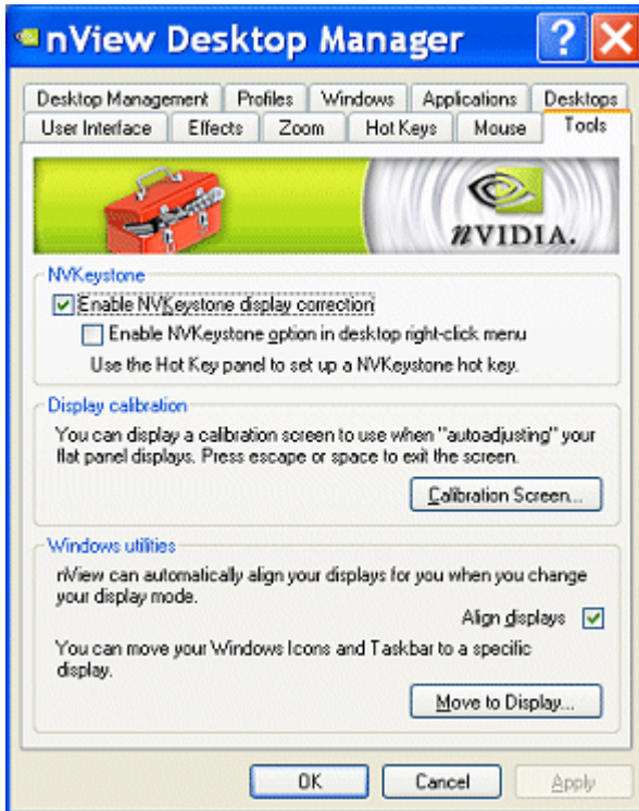
Figure 14.1 Tools Page
