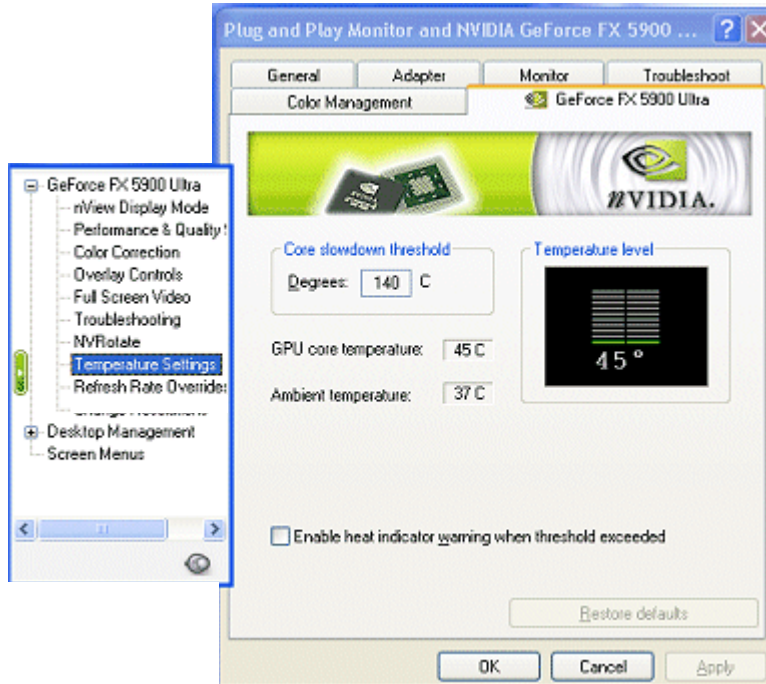
Figure 8.23 Temperature Settings
