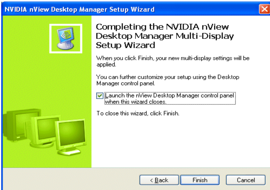
Figure 5.17 Wizard Completion
