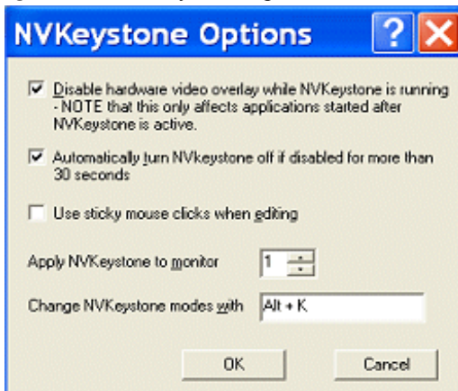
Figure 14.4 NVKeystone Options
