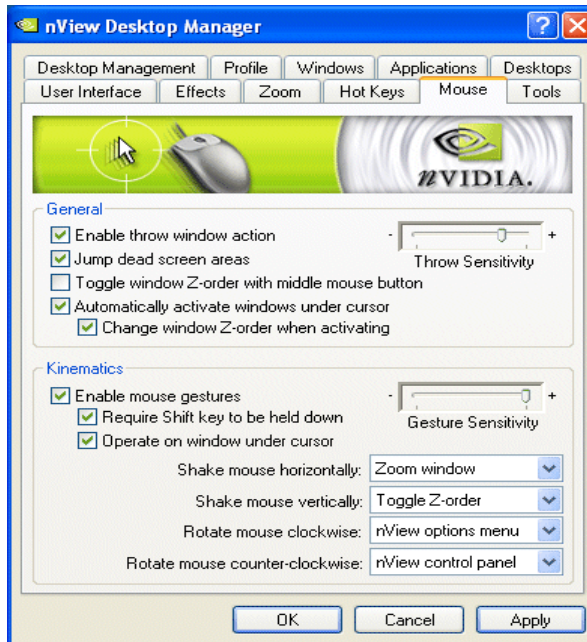
Figure 13.1 Mouse Page 1
