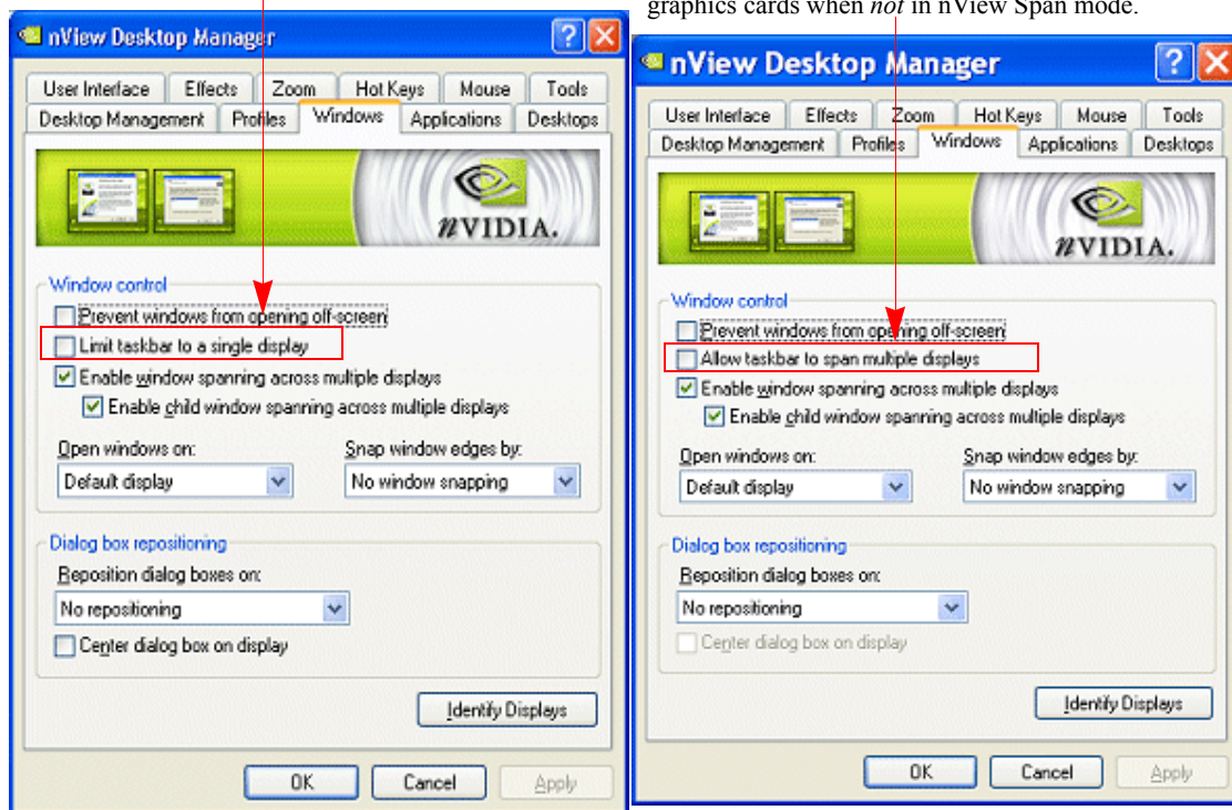
Figure 7.1 Windows Page
