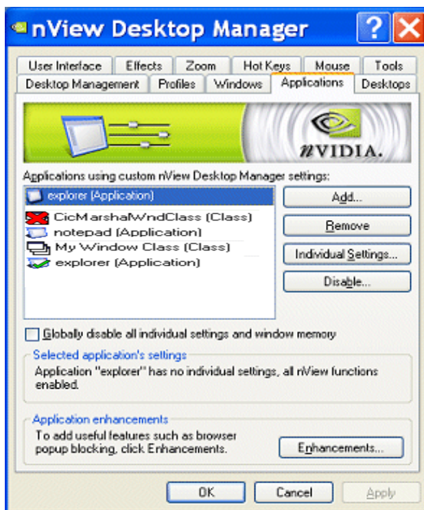
Figure 15.1 Applications Page
